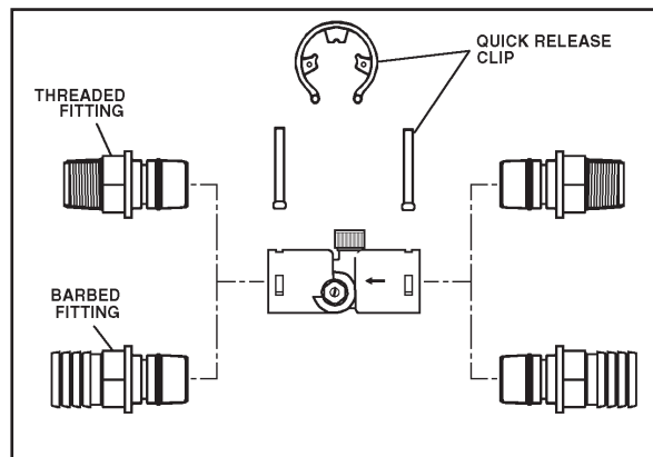
Figure 2: HYDRO-CHARGER INSTALLATION
